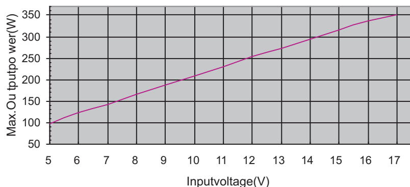
iCharger208B:MAX.OUTPUTPOWERvs.INPUTVOLTAGE
